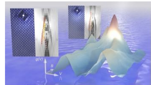
Magnetic-field induced Lifshitz transition observed in tunneling spectra and quasi-particle interference in \text{Sr}_3\text{Ru}_2\text{O}_7 .
