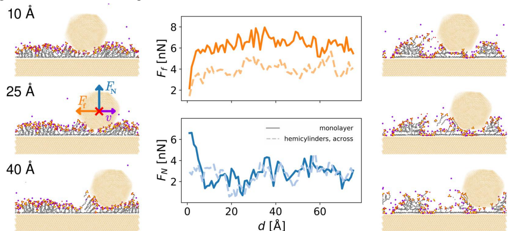
Figure 1: Friction F_f (top, center) and load F_N (bottom) felt by AFM tip (radius r = 25 Å) during initial sliding phase on SDS monolayer (solid lines in plot and conceptual sketch on the left) and across hemicylinders (dashed lines, right sketch) at surface packing density n = 3 \text{ nm}^{-2} , fixed surface–surface distance a = 10 Å and velocity v = 10 \text{ m s}^{-1} . Labels in left hand side conceptual sketch indicate laterally travelled distance d for each snapshot.
