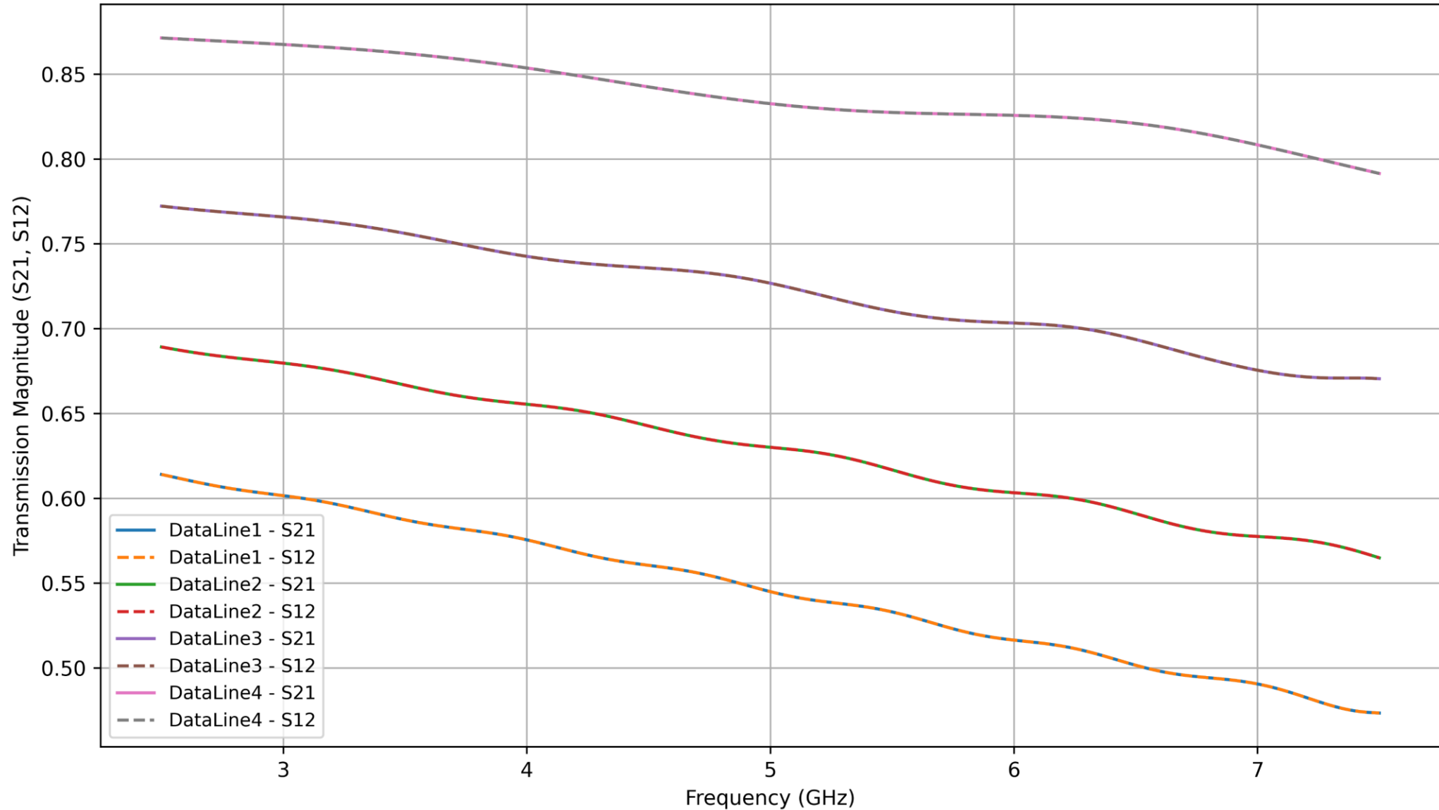
Comparison of Transmission Magnitude of Data Lines in IZM Structure
