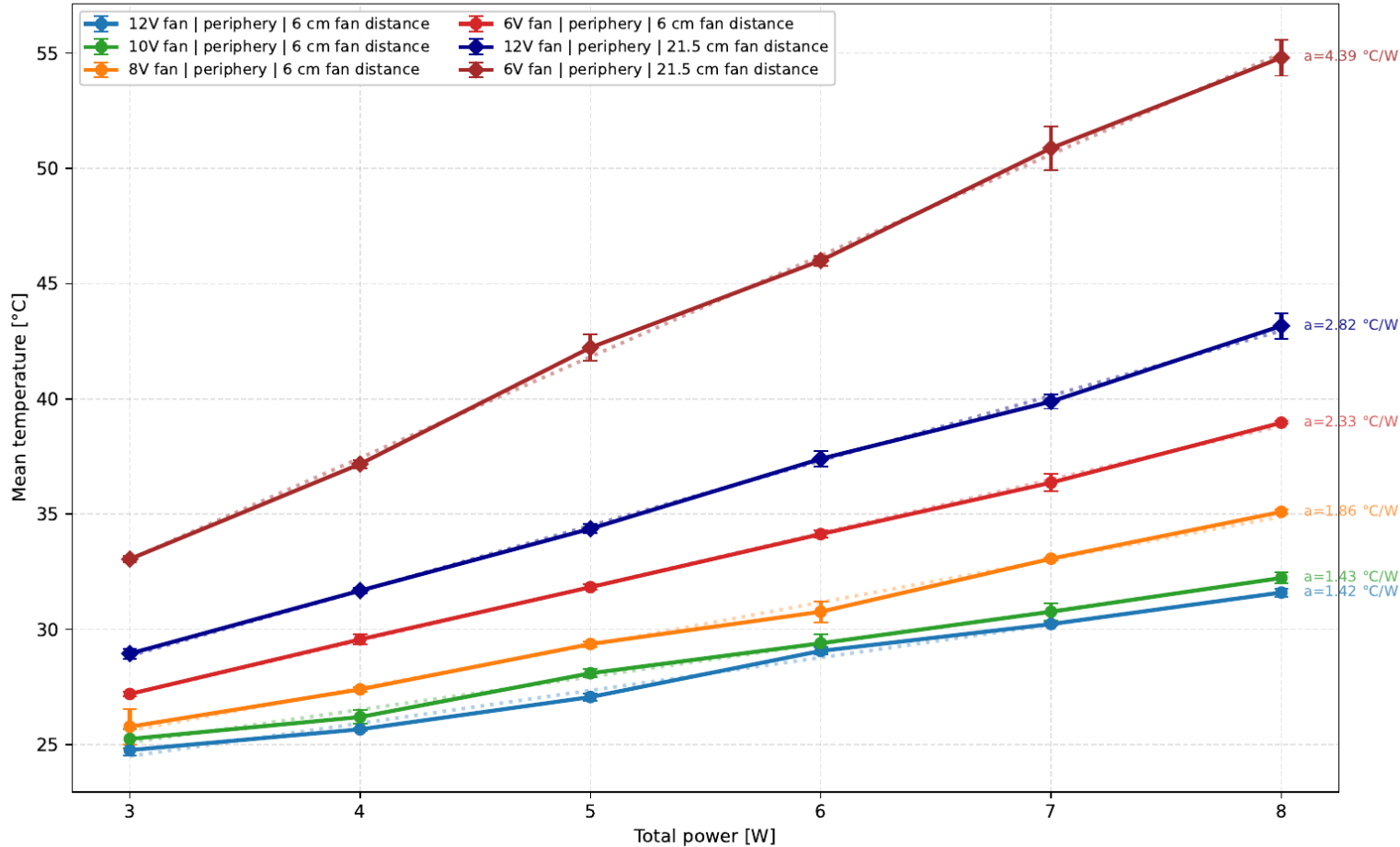
Mean temperature vs power with fits (cooling performance)
